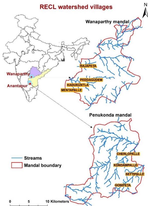
Figure 1. RECL-ICRISAT watershed project sites in Wanaparthy (Telangana) and Anantapur (Andhra Pradesh).
