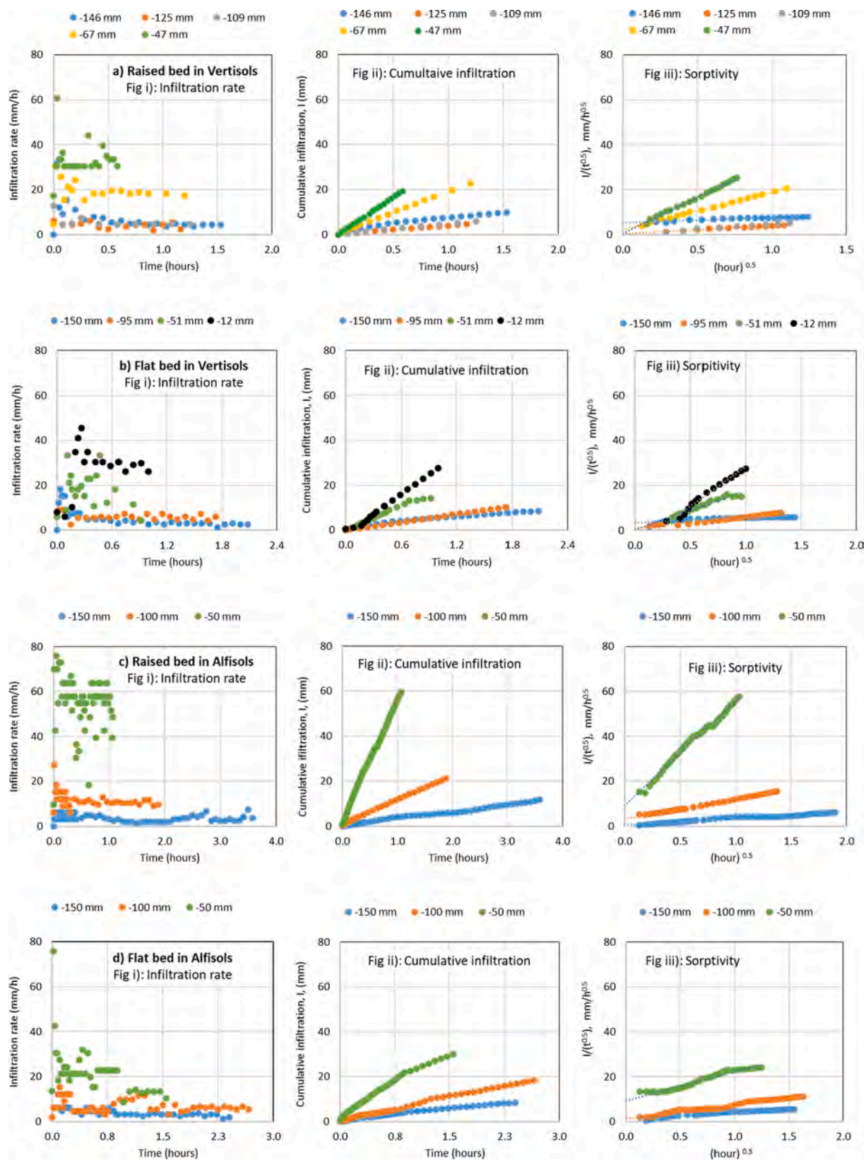
Fig. 3. Infiltration rate, cumulative infiltration and sorptivity for selected TDI experiments in Vertisols and Alfisols.
